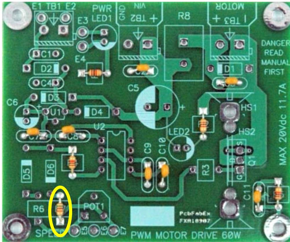
Figure 8: Board with 5.1K resistor installed.
