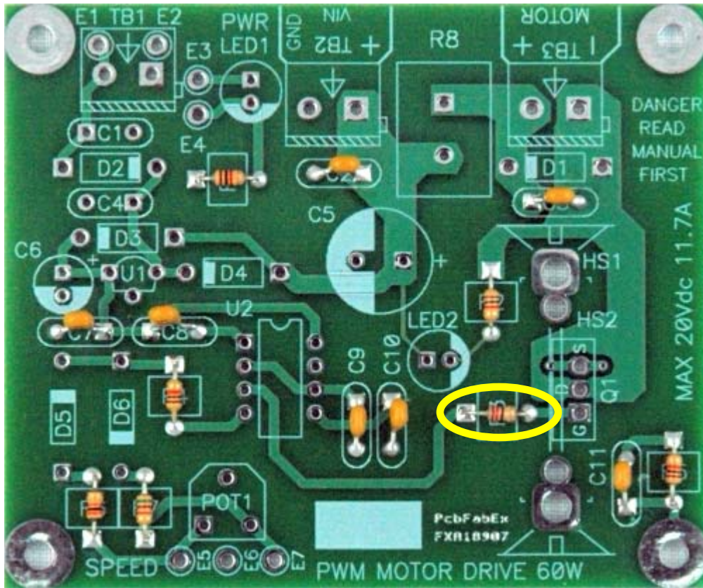
Figure 10: Board with 120 ohm resistors installed.
