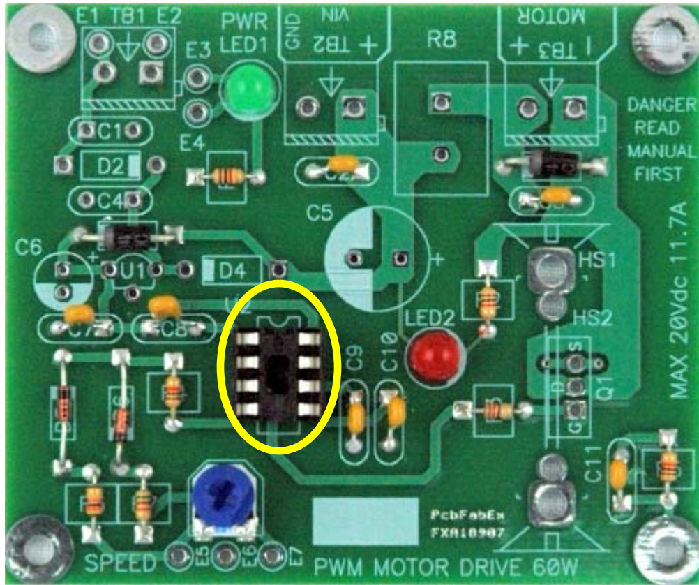
Figure 16: Board with socket and 555 timer installed.
