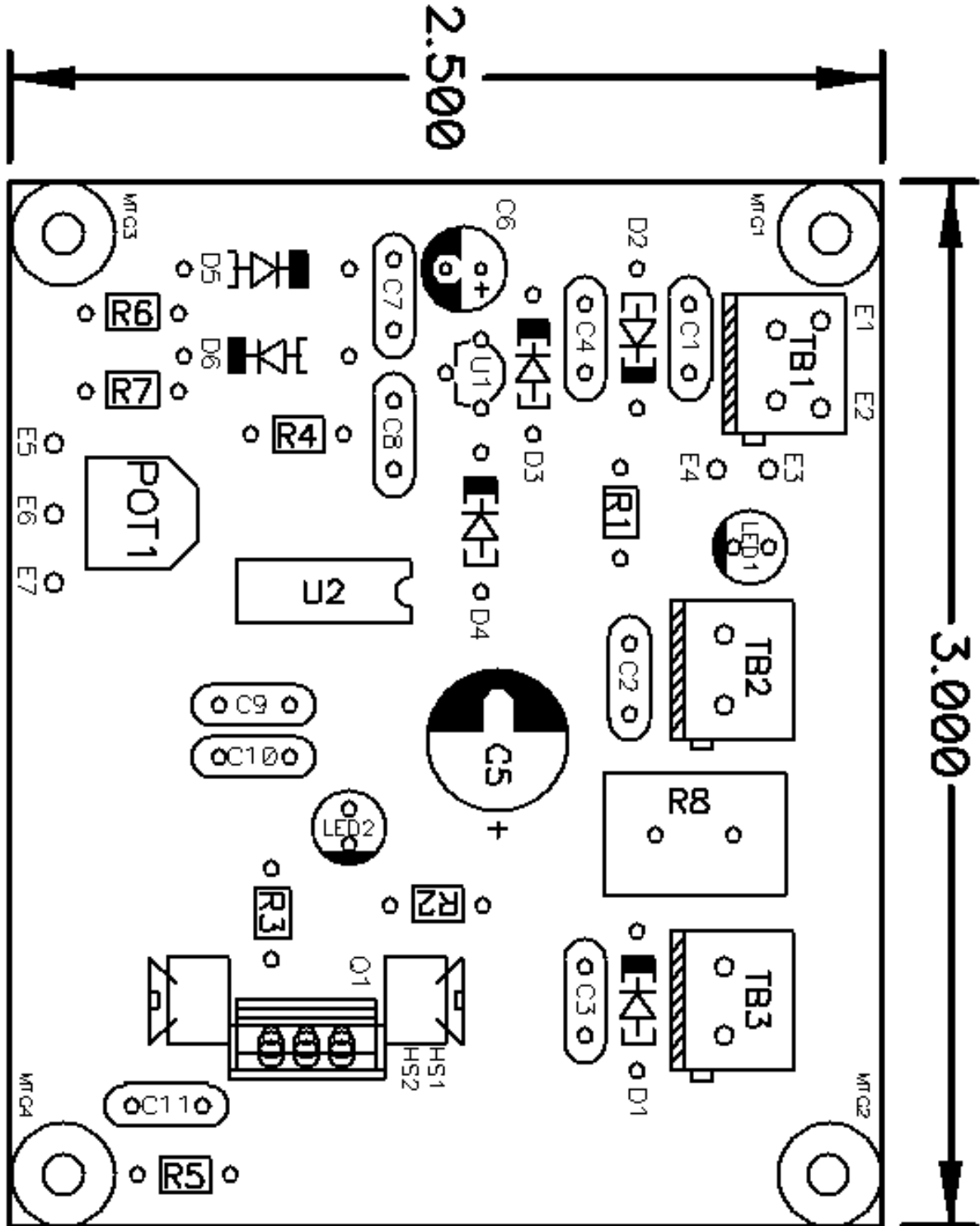
Figure 1: Component Locations and Reference Designators. Board rotated 90 degrees.
