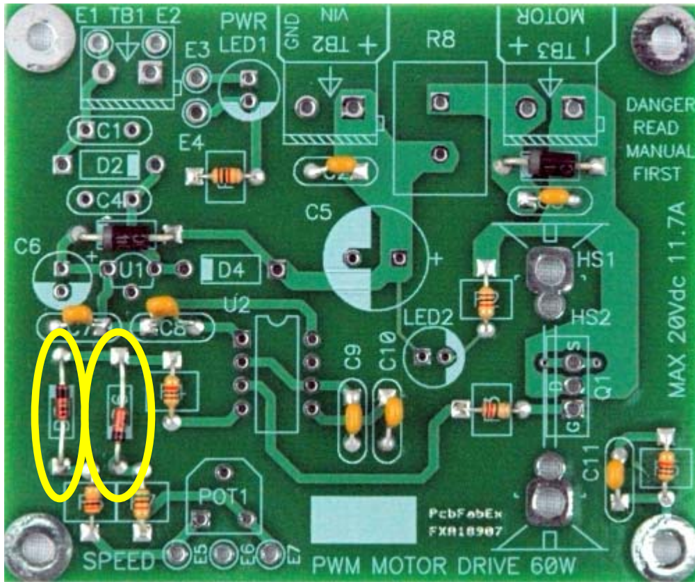
Figure 12: Board with 4148 switching diodes installed.
