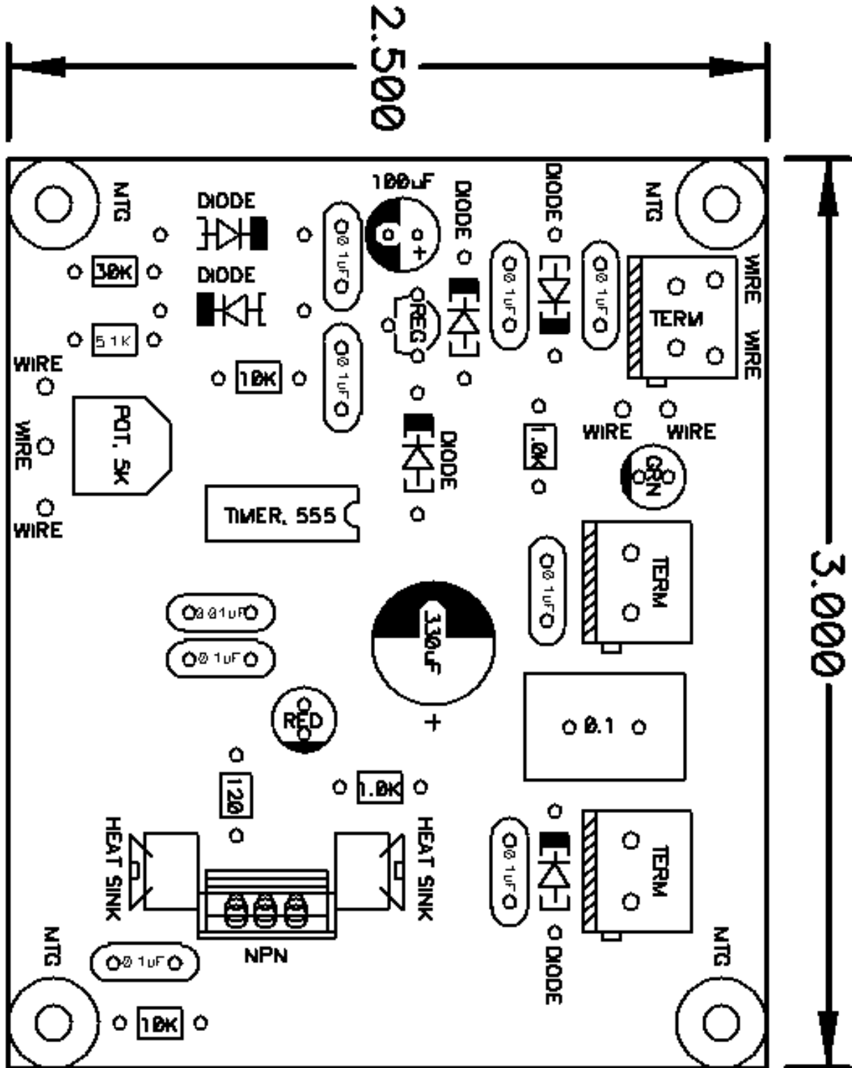
Figure 2: Component Values. Board rotated 90 degrees.
