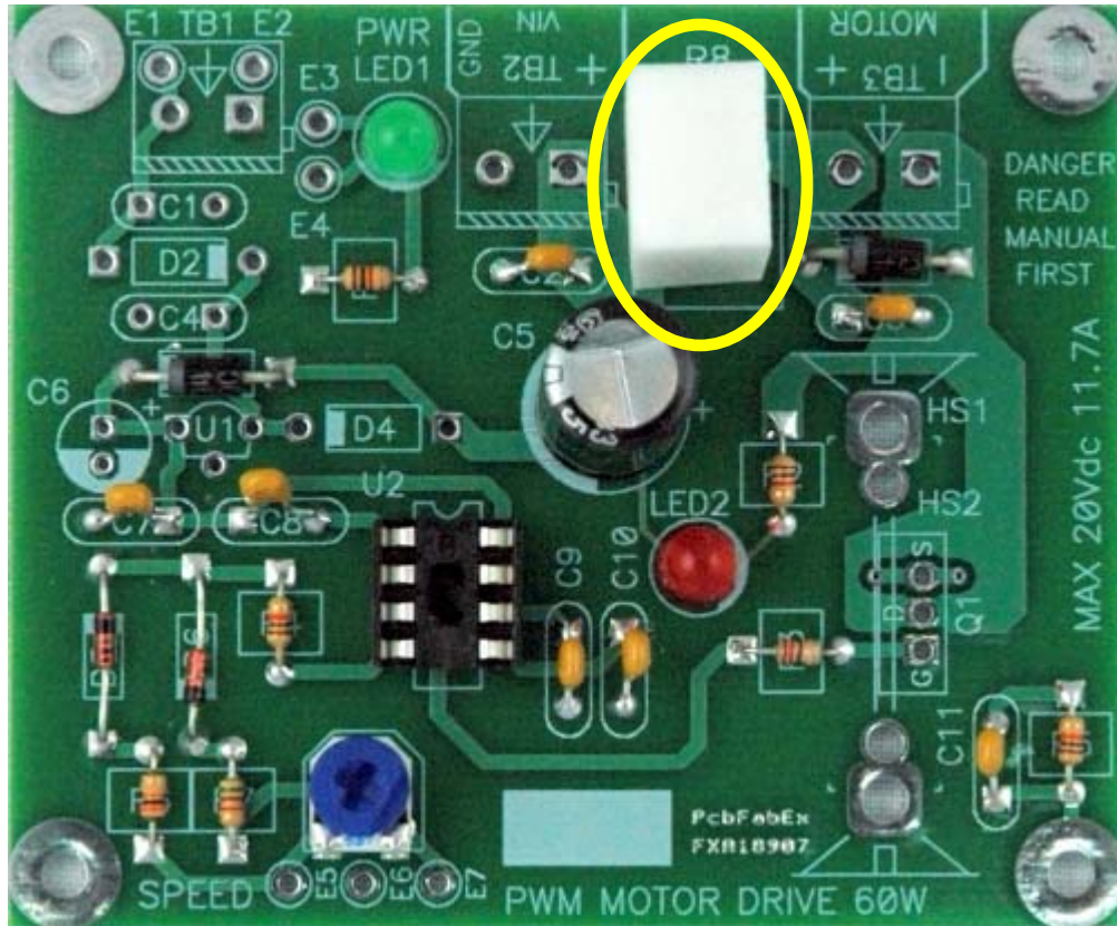
Figure 18: Board with 0.1 ohm resistor installed.
