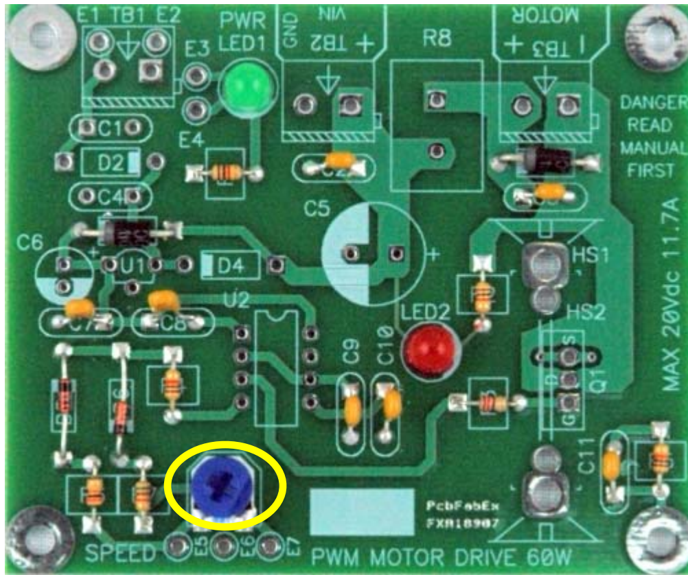
Figure 15: Board with potentiometer installed.
