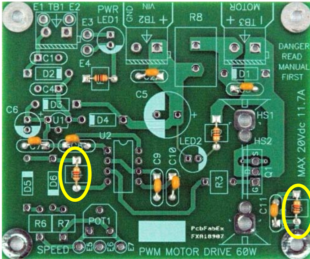
Figure 7: Board with 10K resistors installed.
