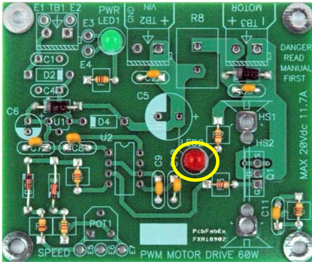
Figure 14: Board with red LED installed.
