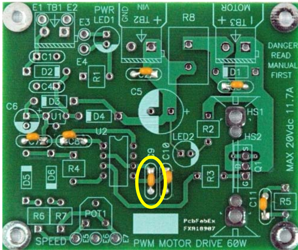
Figure 5: Board with 0.01uF capacitor installed.
