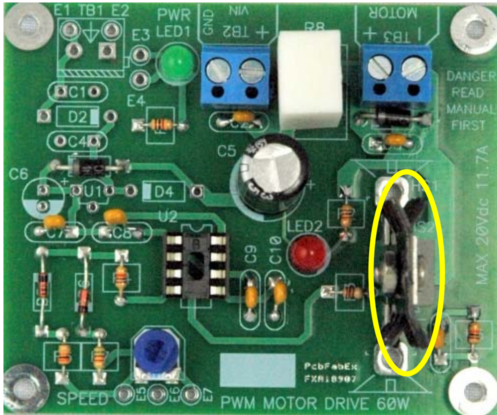
Figure 21: Board with heat sink installed.
