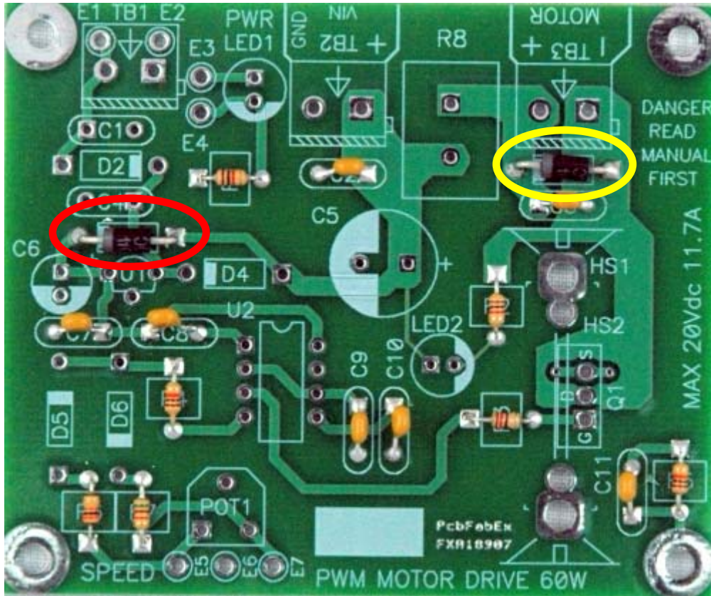
Figure 11: Board with 400V, 1A general-purpose diodes installed. From the kit, locate 2 pieces of the 400V, 1A general-purpose diodes.
