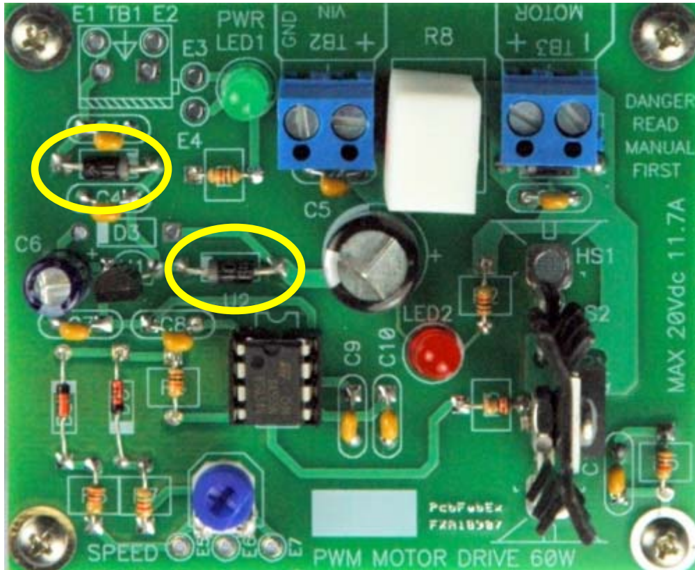
Figure 25: Board with 400V, 1A general-purpose diodes installed.
