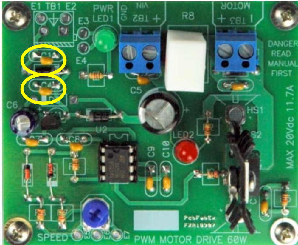
Figure 23: Board with 0.1uF ceramic capacitors installed.
