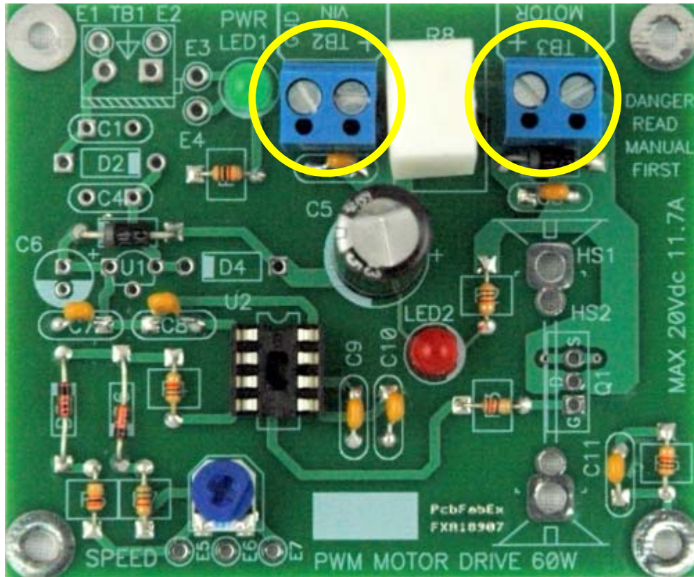
Figure 19: Board with terminal blocks installed.
