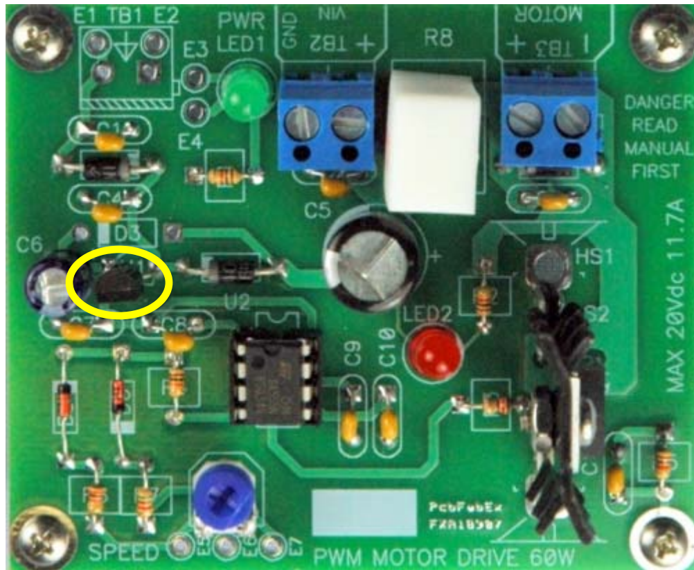
Figure 24: Board with 5V regulator installed.
