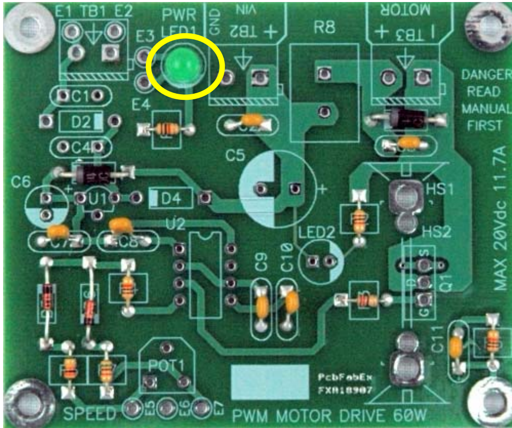
Figure 13: Board with green LED installed.
