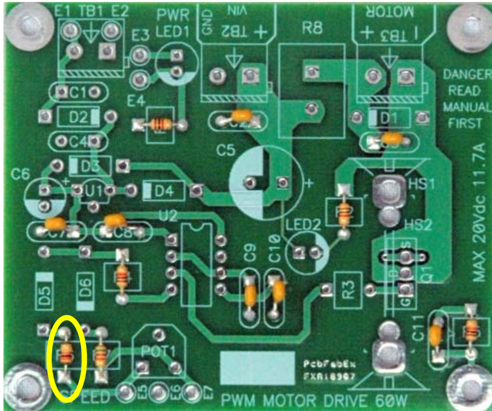
Figure 9: Board with 30K resistor installed.
