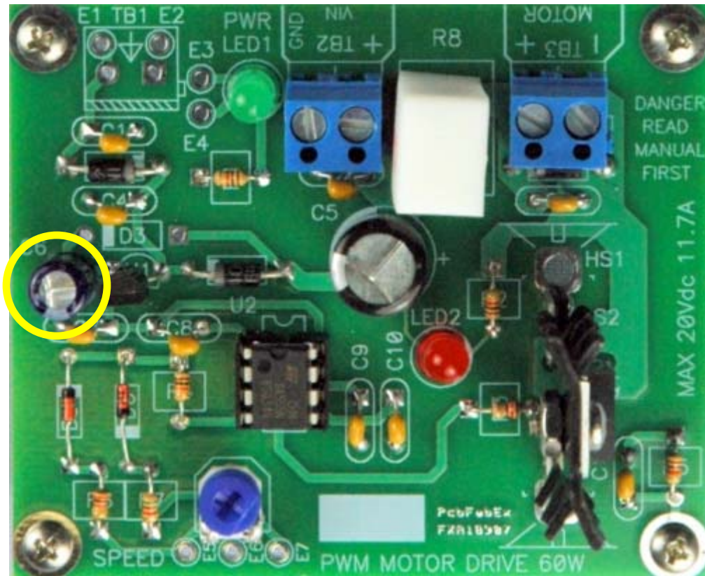
Figure 22: Board with aluminum electrolytic capacitors installed.
