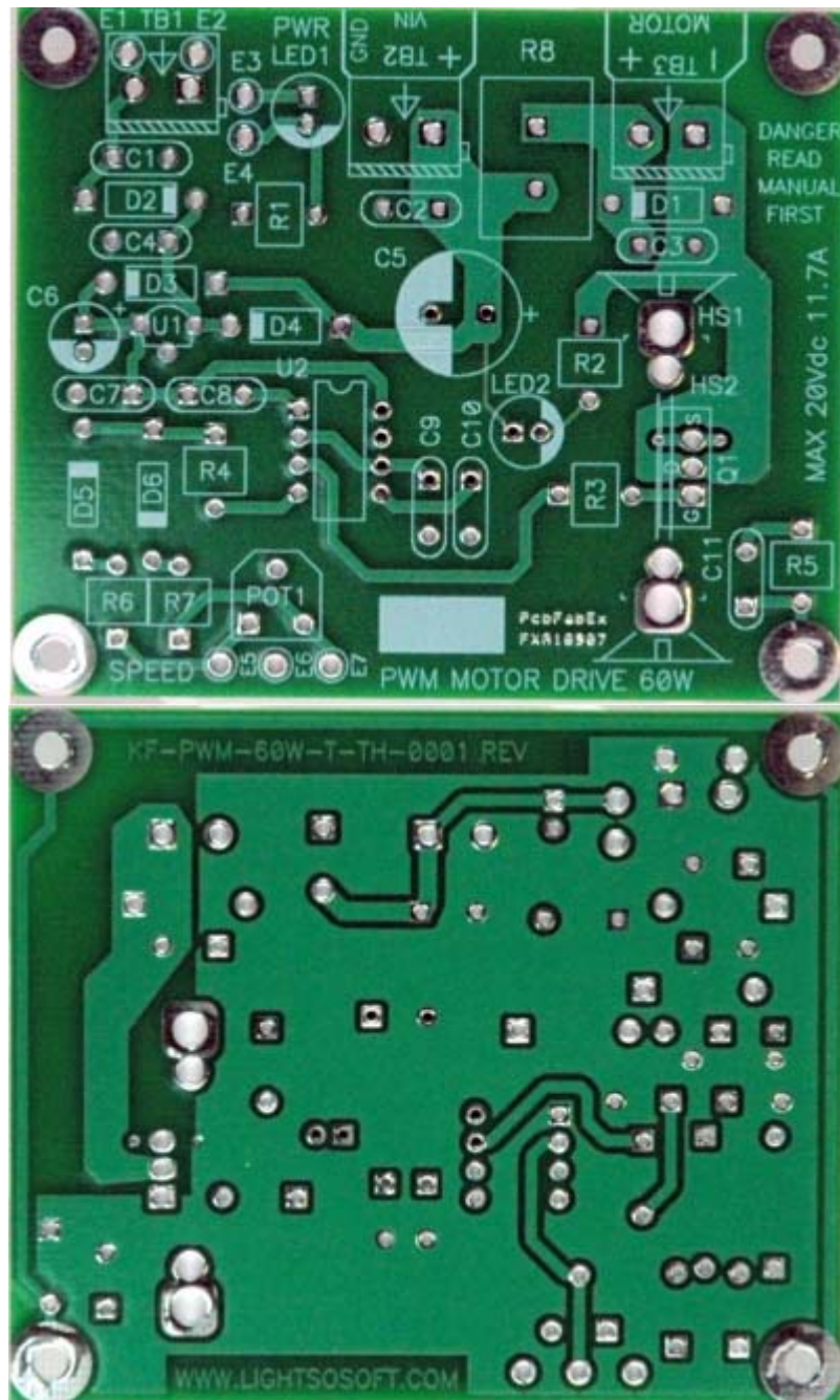
Figure 3: Board with no components installed, top and bottom sides.
