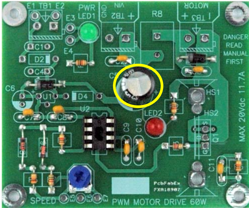
Figure 17: Board with aluminum electrolytic capacitors installed.
