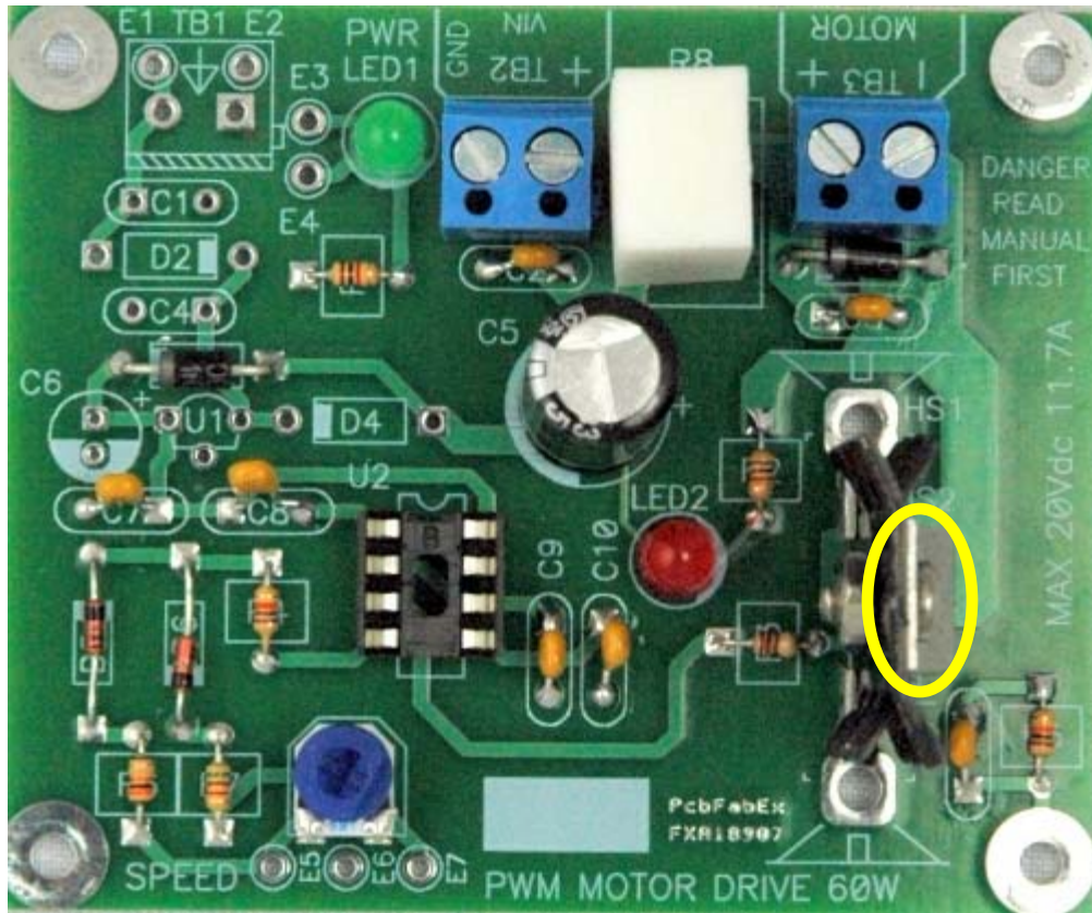
Figure 20: Board with MOSFET installed.
